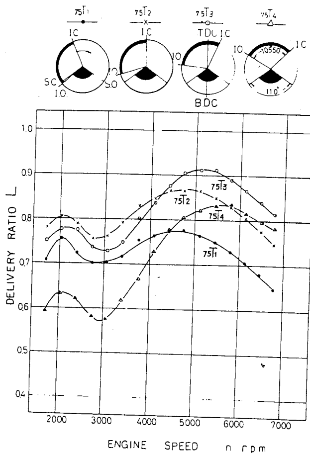
Fig. 4 (b) - Relation between delivery ratio and engine speed, 75 deg valve cut-angle
