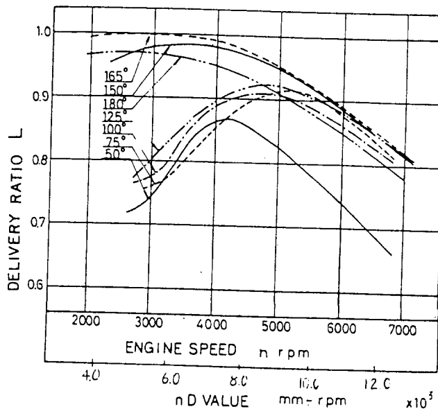
Fig. 5 - Relation between delivery ratio and engine speed. Envelopes from Figs. 4 a-g give limiting delivery ratio curve
