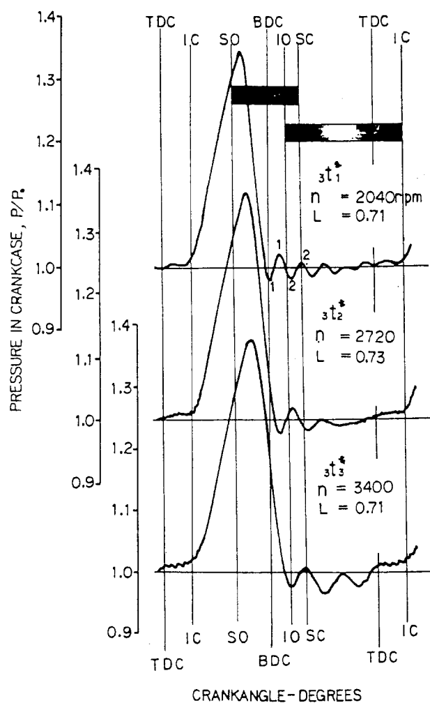
Fig. 16 - Crankcase indicator diagrams, case of 165T_3 (without cylinder head)
