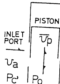
Fig. 39 - Relation between inlet velocity and piston velocity
