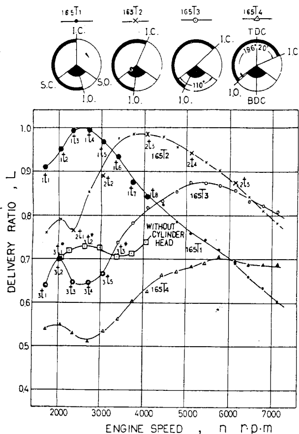
Fig. 4 (f) Relation between delivery ratio and engine speed, 165 deg valve cut-angle. Notations 1^1-7^1 2^1-5^1 3^1-5 , 3^1-3 correspond to each indicator diagram in Figs. 9, and 12-16
