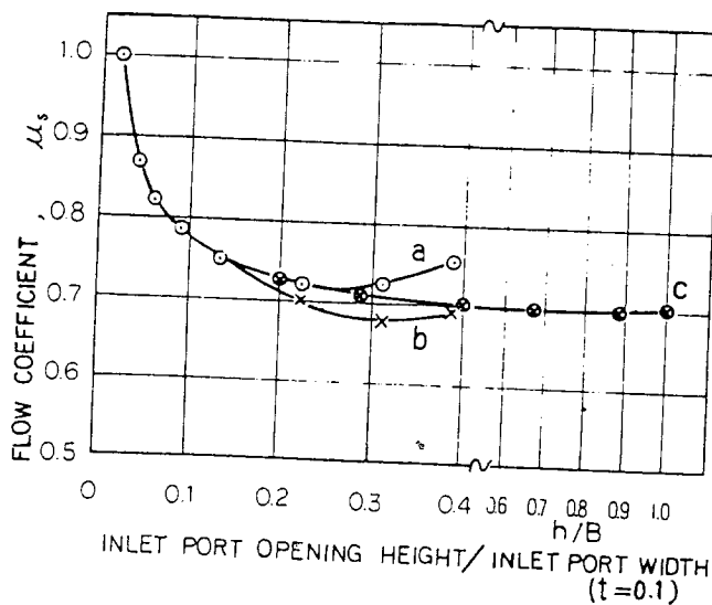
Fig. 34 - Relation between the flow coefficient and inlet port configuration (relation between cylinder liner inlet port and model of inlet port)
