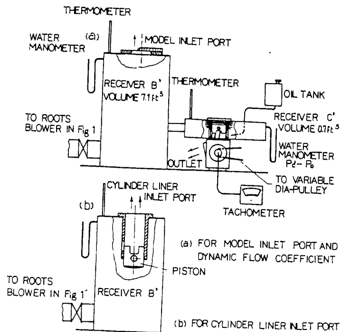
Fig. 30 - Test equipment used for measuring the flow coefficient of inlet port
