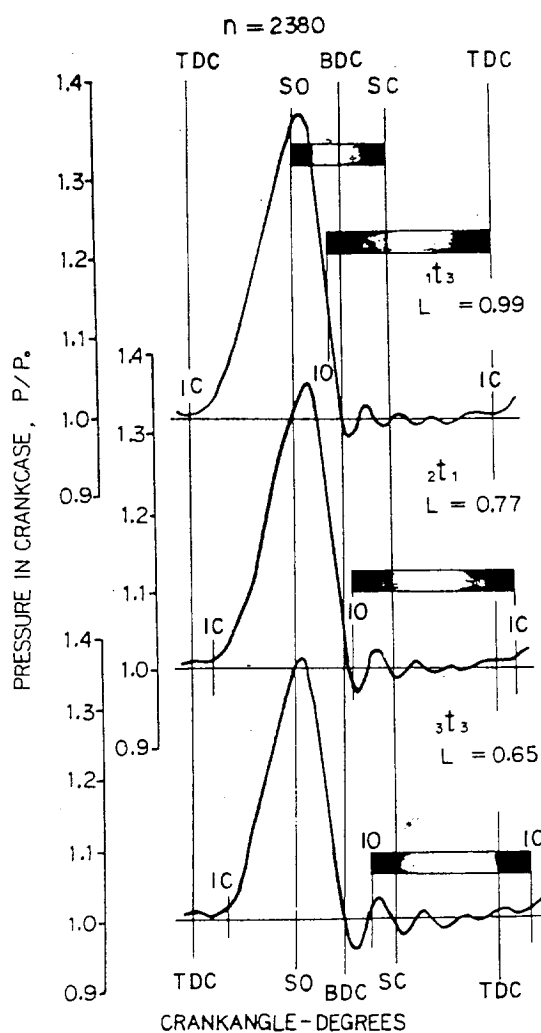
Fig. 13 - Crankcase indicator diagrams, cases of 165T_1 , 165T_2 and 165T_3
