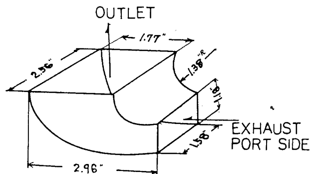
Fig. 20 - Exhaust duct in detail
