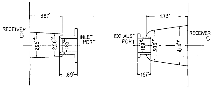
Fig. A-2 - Inlet and exhaust ducts in detail
