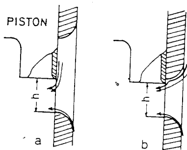
Fig. 33 - Influence of rounded upper edges on inlet flow
