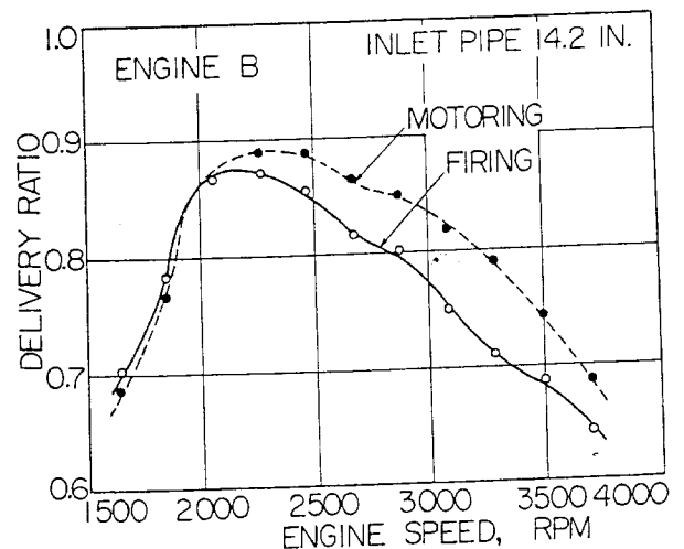
Fig. 14 - Comparison of motoring and firing delivery ratio
