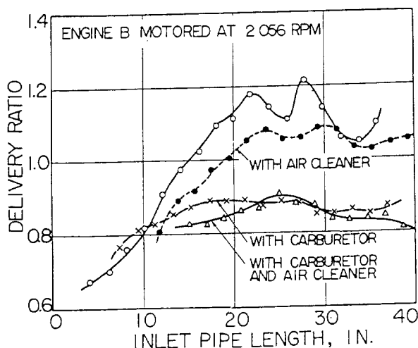
Fig. 24 - Effect of carburetor and air cleaner
