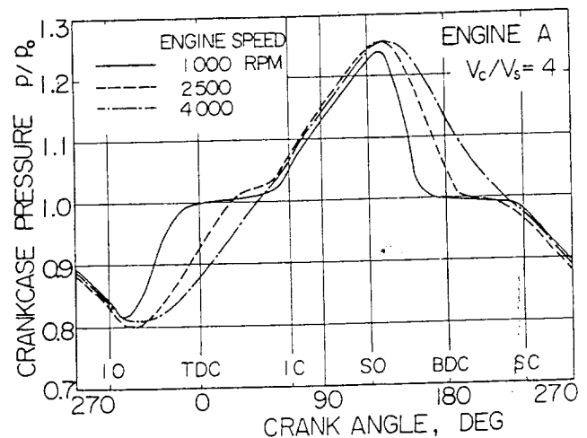
Fig. 2 - Calculated variation of crankcase pressure
