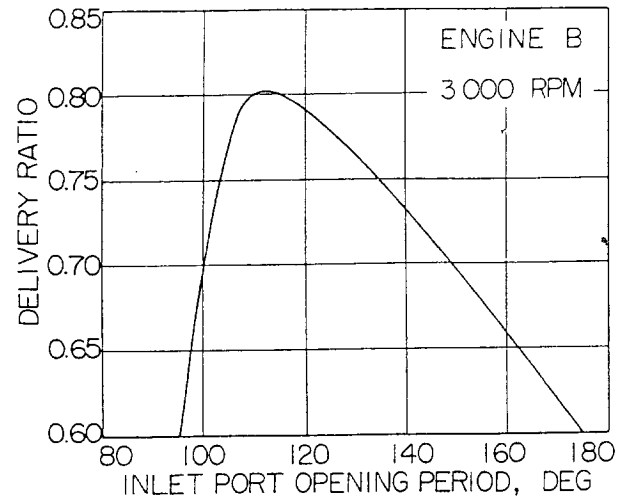
Fig. 19 - Effect of inlet port opening period (calculated)
