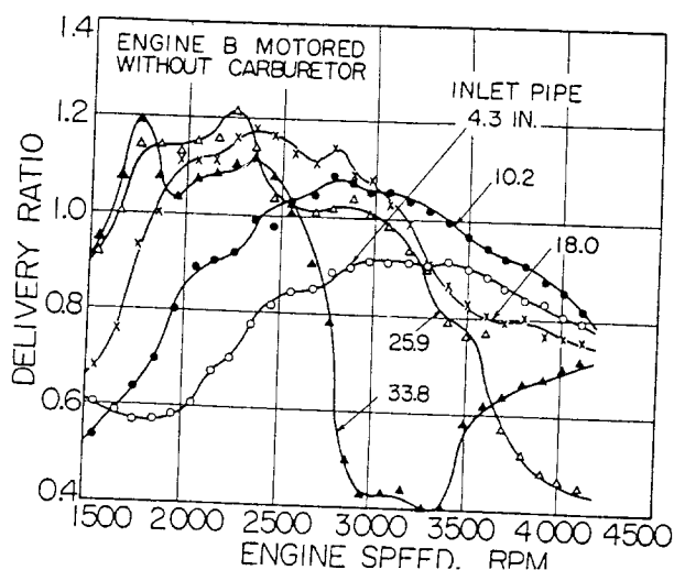
Fig. 15 - Effect of inlet pipe length
