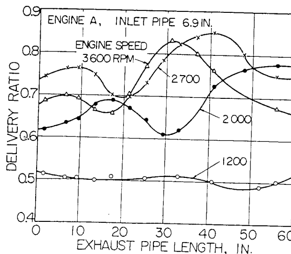
Fig. 11 - Effect of exhaust pipe length
