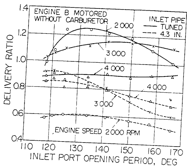
Fig. 21 - Effect of inlet port opening period
