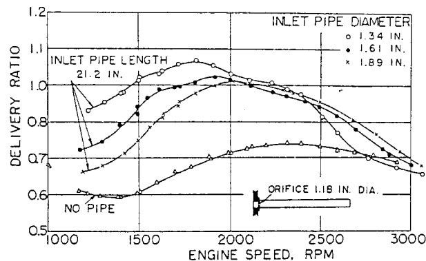
Fig. D - Effect of throttling
