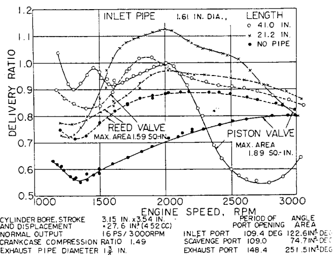
Fig. B - Comparison between reed valve and piston valve
