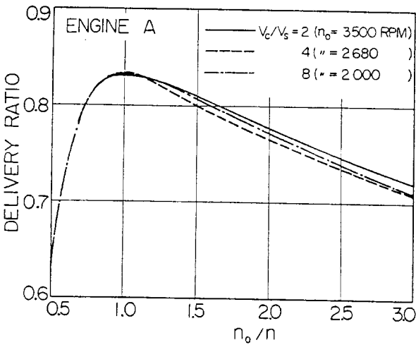
Fig. 4 - Relationship between delivery ratio and ratio of engine speed n_o , giving a maximum delivery ratio to en-
