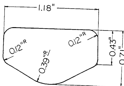
Fig. 17 - Engine B inlet port dimensions
