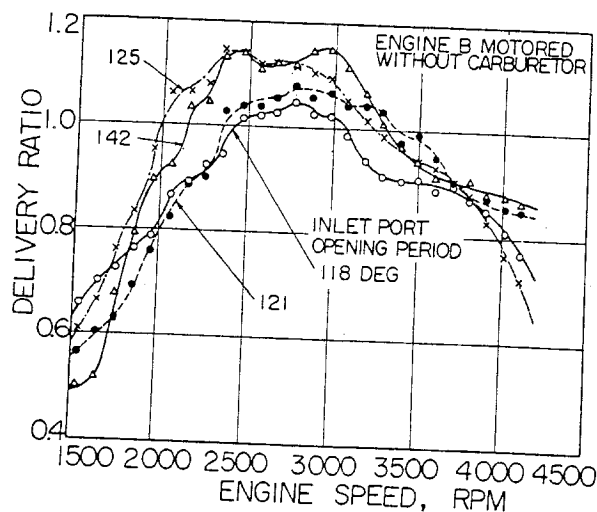
Fig. 22 - Delivery ratio for inlet pipe selected to produce highest possible delivery ratio at 3000 rpm
