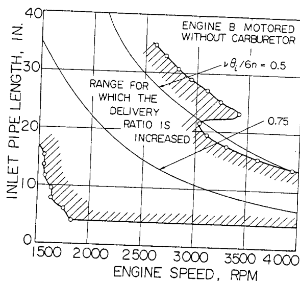
Fig. 16 - Range of inlet pipe lengths for which delivery ratio is higher than that for shortest length (4.3 in.)
