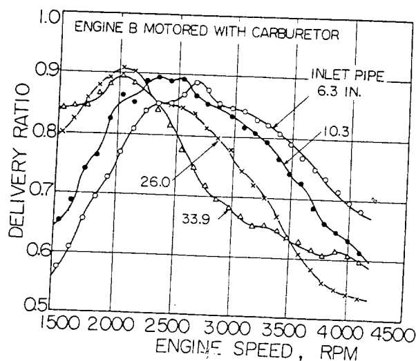
Fig. 23 - Effect of inlet pipe length with carburetor installed
